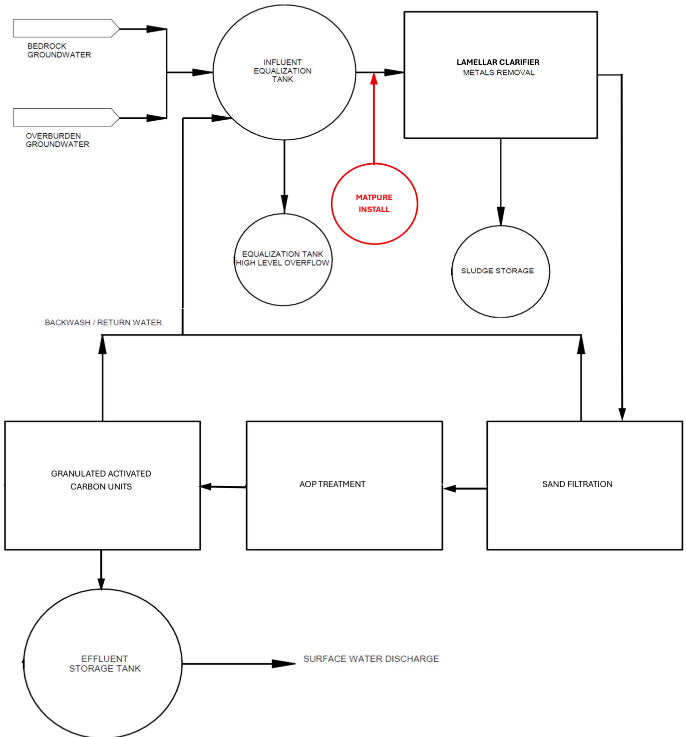
Figure 1: Referred Groundwater Treatment Design with AOP/GAC finishing.
