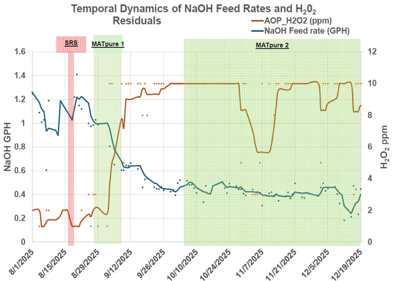
Figure 2: Temporal Dynamics of NaOH Feed Rates and H 2 O 2 Residuals
