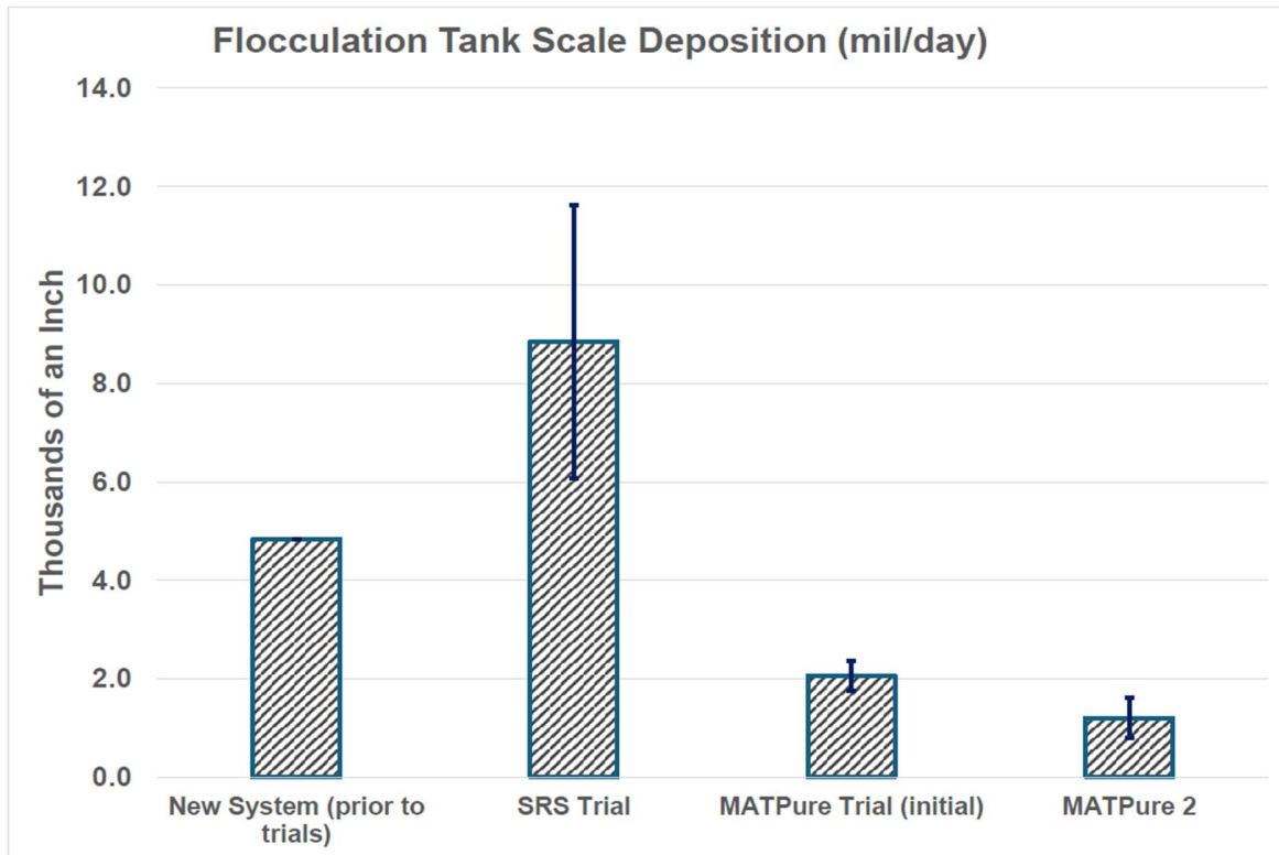
Figure 4: Flocculation Tank Scale Deposition Rate.
