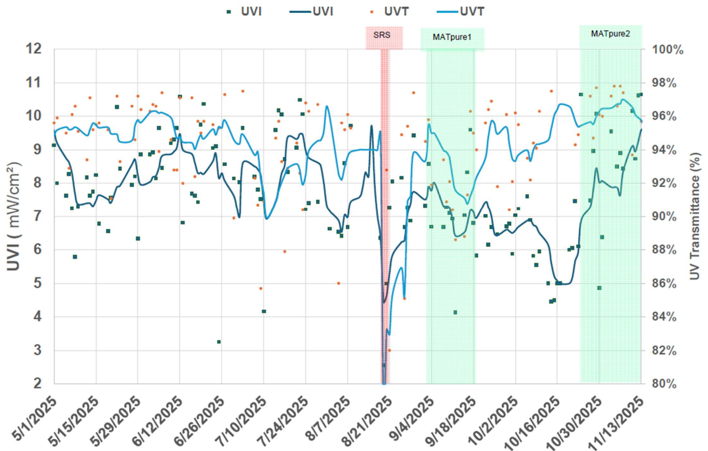
Figure 3: Dynamics of UV Transmittance and UV Intensity
