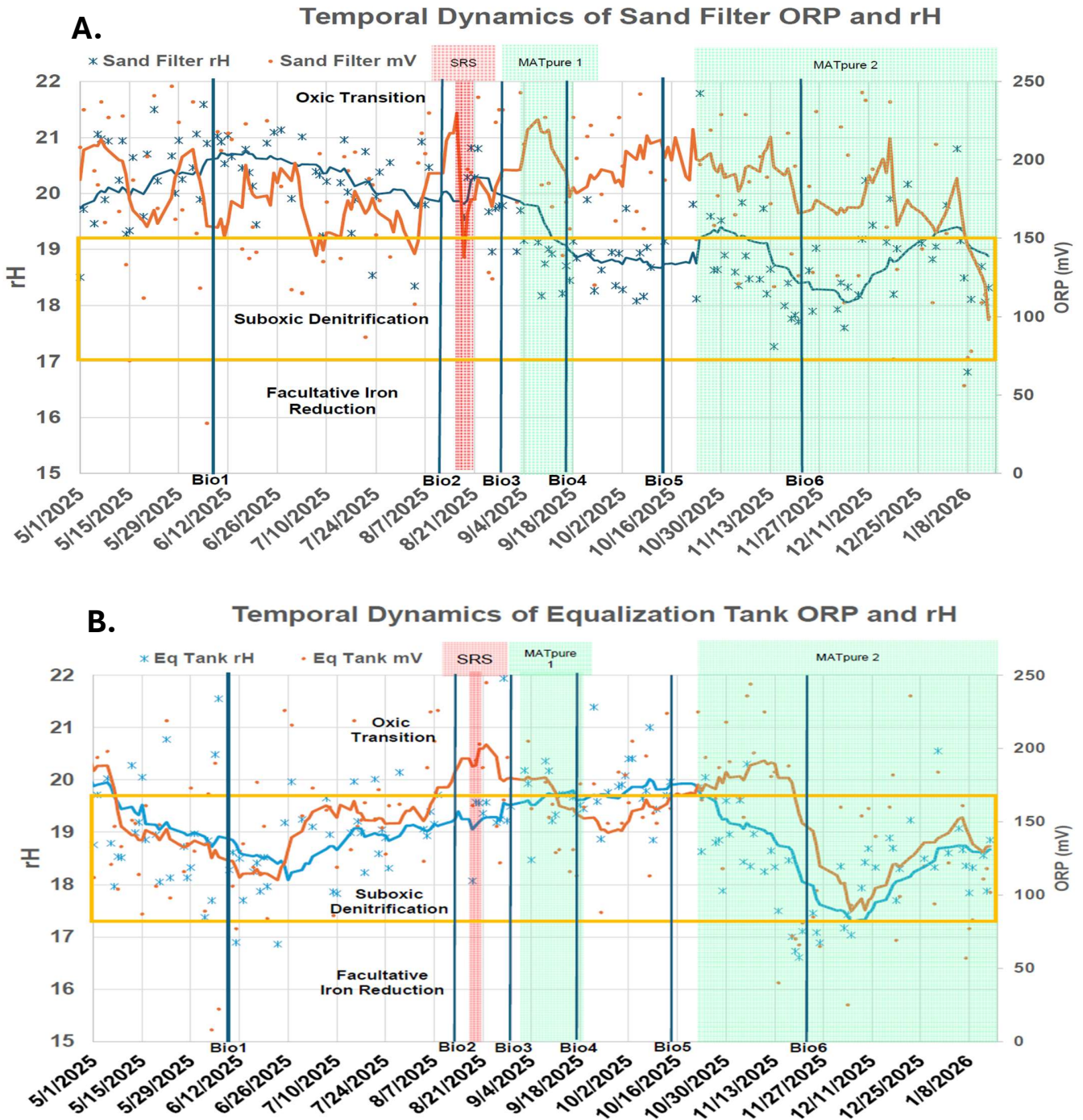
Figure 7: EQ ORP and rH Temporal Dynamics Influence in Sand Filter and Backwash Recycling The groundwater treatment system was configured to continuously return sand filter backwash to the EQ basin. Catalytic water conditioning applied downstream of the EQ progressively influenced the sand filter and its backwash (A). EQ electrochemical conditions also changed gradually via the influence of recycled backwash, versus baseline (backwash) and influent (well) seeding alone (B). Within relatively short operational periods, resultant MATpure® treated sand filter and EQ water accumulated pronounced shifts in EQ rH and ORP measurements. These measurements indicate that catalytic water stabilization effects persisted through coagulation, clarification, and subsequent sand filter (permeate/backwash) treatment and were partially retained upon recycle to the EQ basin.
